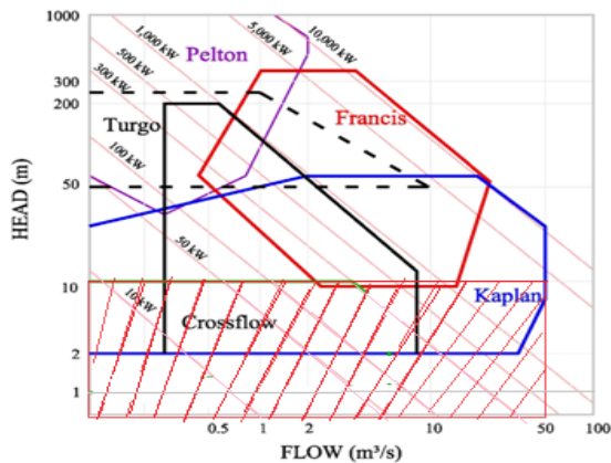
Fig. 2. Hydro-turbines characteristics in terms of water head and flow rate [14]
