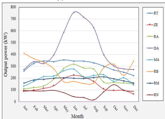
(b)Kaplan turbine
