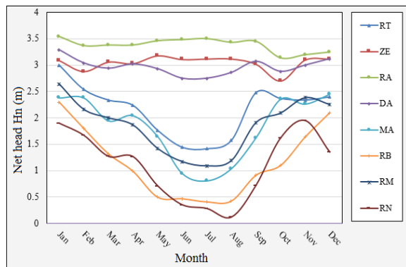
Fig. 5. The net head for the selected sites
