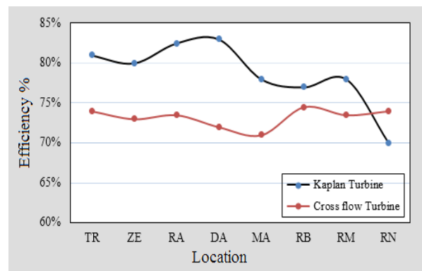
Fig. 7 Efficiency of the Kaplan and Cross flow hydro-turbine at each location
