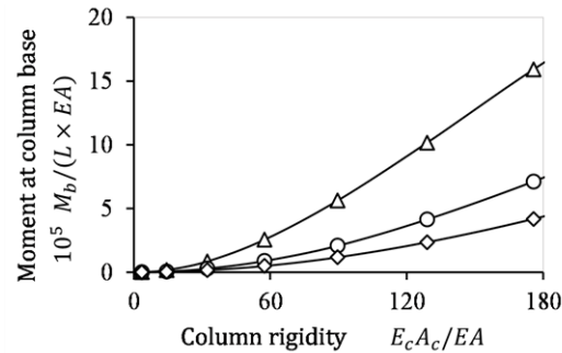
Fig. 45. Variation of moments at column base with columns stiffness
