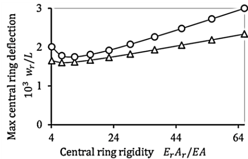
Fig. 27. Variation of central ring deflections with central rings stiffness and diameters ratio.
