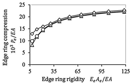
Fig. 37. Variation of edge ring compression forces with edge ring stiffness and load intensity.
