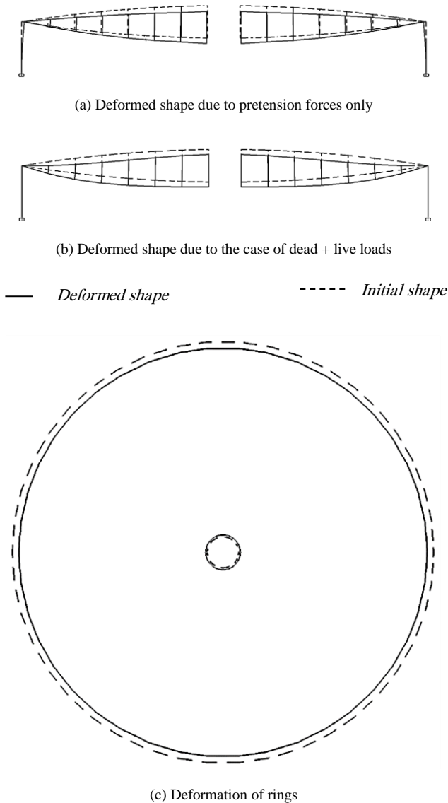
Fig. 4. Illustrative sketches of the deformed structure
