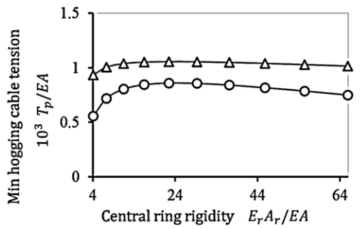
Fig. 30. Variation of hogging cable tensions with central rings stiffness and diameters ratio.
