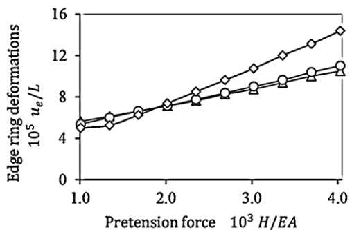
Fig. 24. Variation of edge ring deformations with cable pretension forces
