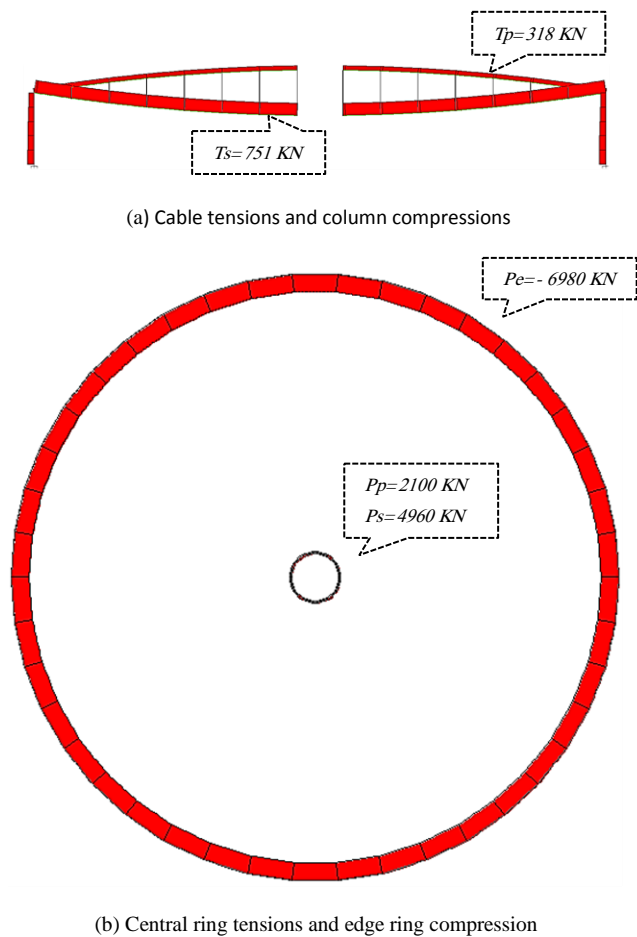
Fig. 5. Sketches of normal forces due to the case of dead + live loads
