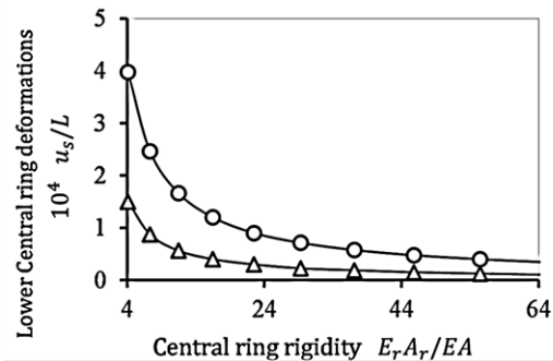
Fig. 28. Variation of lower central ring deformations with central rings stiffness and diameters ratio.
