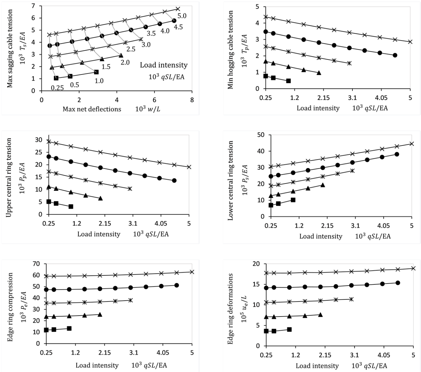
Fig. 47. Response of the convex cable roof beams, for sag/rise to span ratio f=4\% L , load intensity qSL/EA=0.25 \times 10^{-3} to 5 \times 10^{-3} , pretension force H/EA=1 \times 10^3 to 5 \times 10^3 , and edge ring rigidity EeAe/EA=167 .
