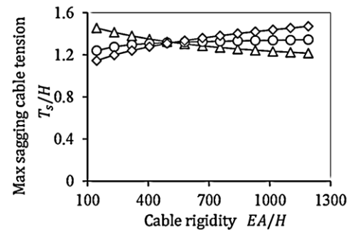
Fig. 16. Variation of sagging cable tensions with cable sizes
