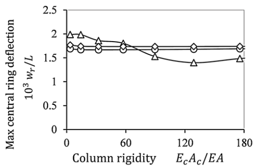
Fig. 40. Variation of central ring deflections with columns stiffness
