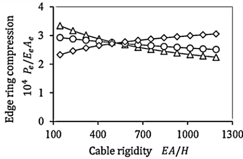
Fig. 19. Variation of edge ring compression forces with cable sizes
