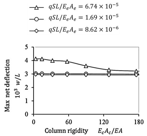
Fig. 39. Variation of net deflections with columns stiffness
