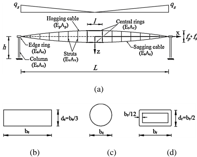
Fig. 3. Convex cable beam structure: (a) Cross section through the roof; (b) Cross section of the R.C. edge beam; (c) Cross section of the R.C. column; (d) Cross section of the steel central ring.
