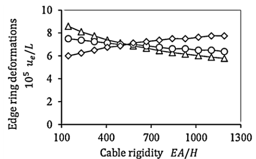
Fig. 18. Variation of edge ring deformations with cable sizes
