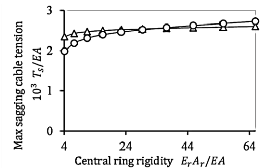
Fig. 29. Variation of sagging cable tensions with central rings stiffness and diameters ratio.
