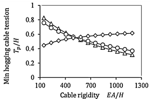
Fig. 17. Variation of hogging cable tensions with cable sizes
