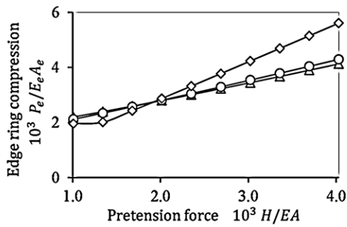
Fig. 25. Variation of edge ring compression forces with cable pretension forces
