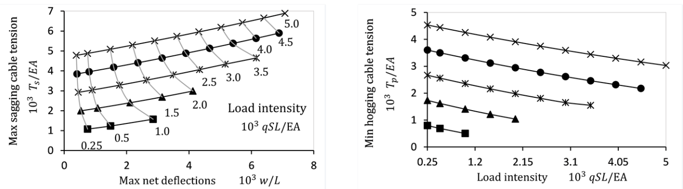
Fig. 48. Response of the convex cable roof beams, for sag/rise to span ratio f=4\% L , load intensity qSL/EA=0.25 \times 10^{-3} to 5 \times 10^{-3} , pretension force H/EA=1 \times 10^3 to 5 \times 10^3 , and edge ring rigidity EeAe/EA=250 .
