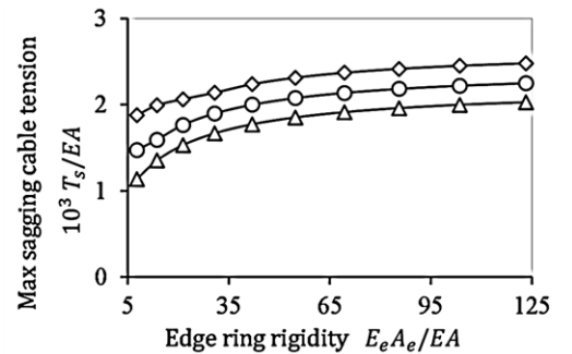
Fig. 34. Variation of sagging cable tensions with edge ring stiffness and load intensity.
