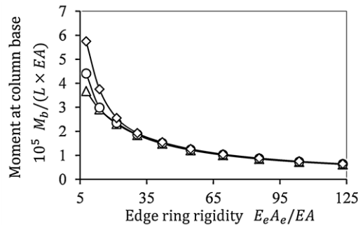
Fig. 38. Variation of moments at column base with edge ring stiffness and load intensity.
