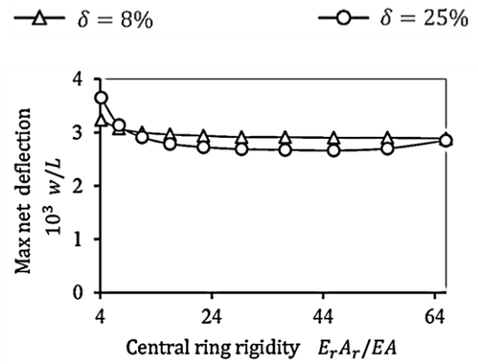
Fig. 26. Variation of net deflections with central rings stiffness and diameters ratio.
