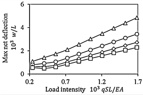
Fig. 6. Variation of maximum net deflections with cables curvature and load intensities
