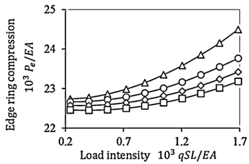
Fig.13. Variation of edge ring compression forces with cables curvature and load intensities
