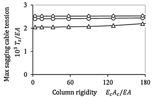
Fig. 41. Variation of sagging cable tensions with columns stiffness
