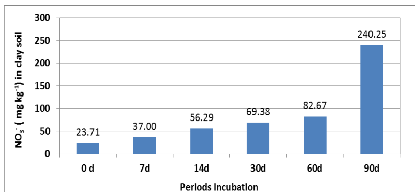
Fig. (2): Effect of incubation periods on the mineralization of nitrogen forms (NO 3 - mg kg -1 ) in clay soil.
