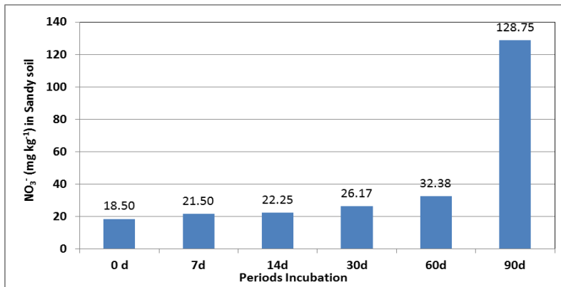
Fig. (4): Effect of incubation periods on the mineralization of nitrogen forms ( NO_3^- \text{ mg kg}^{-1} ) in sandy soil.
