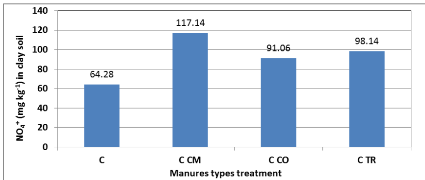
Figs (5): Effect of manure types on the mineralization of nitrogen forms (NH 4 + ) in clay soil.
