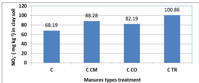
Fig (1): Effect of manure types on the mineralization of nitrogen forms ( \text{NO}_3^- ) in clay soil.
