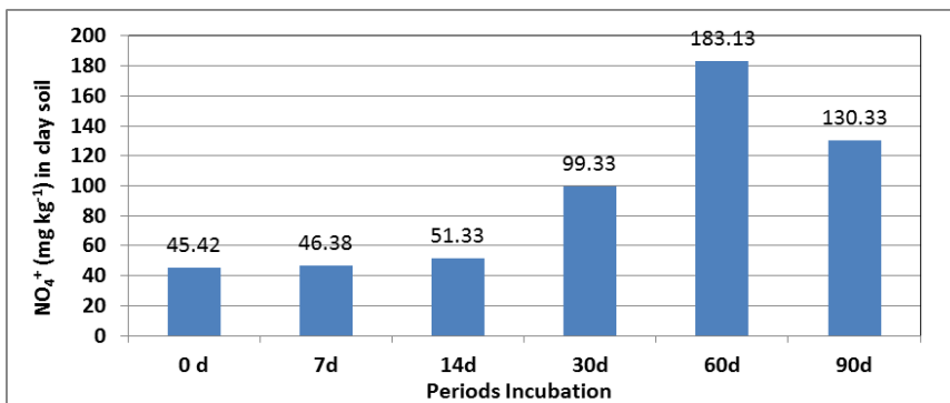
Figs. (6): Effect of incubation periods on the mineralization of nitrogen forms (NH 4 + mg kg -1 ) in clay soil.
