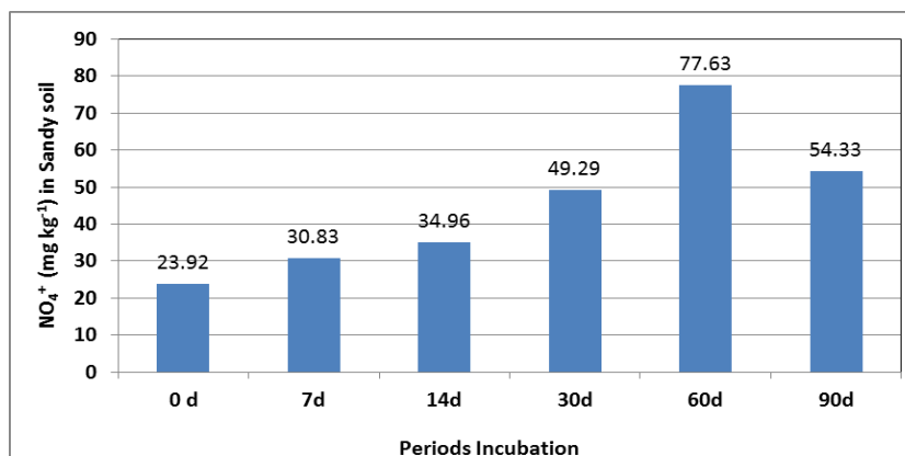
Figs. (8): Effect of incubation periods on the mineralization of nitrogen forms ( \text{NH}_4^+ \text{mg kg}^{-1} ) in sandy soil.
