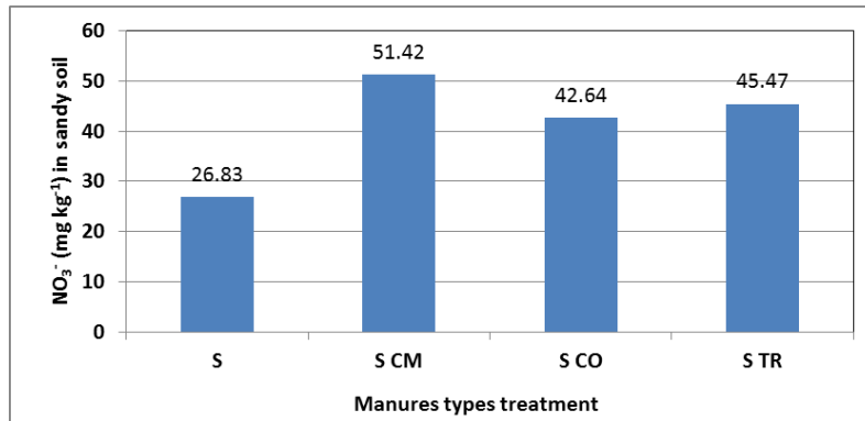
Fig. (3): Effect of manure types on the mineralization of nitrogen forms ( NO_3^- ) in sandy soil.
