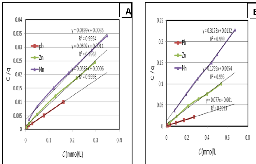
Figure 4: Langmuir adsorption isotherm of Pb^{2+} , Zn^{2+} and Mn^{2+} on apatite mineral (A) mono-metal and (B) ternary-metal
