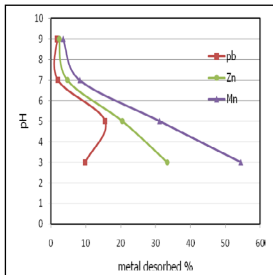
Figure 8: Percentage of metal desorption as a function of pH
