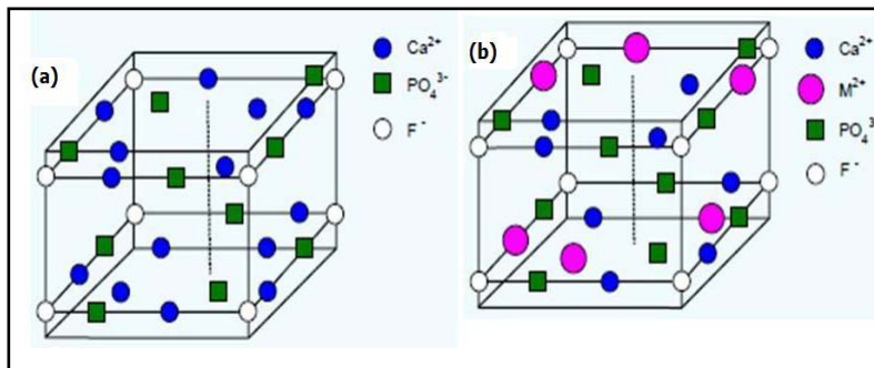
Figure 6: Unit cell of apatite mineral (a) before and (b) after interaction with heavy metal ions ( M^{2+} ) (after Sona Saxena and Disouza, 2006)
