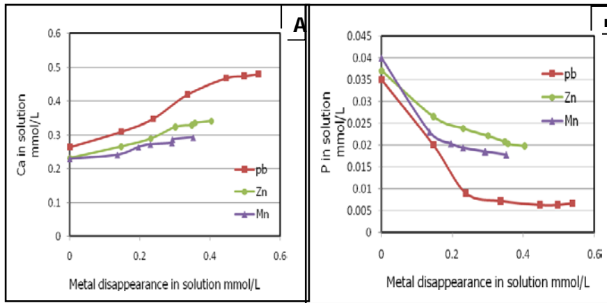
Figure 5: Calcium (A) and Phosphate (B) in equilibrium solution as a function of heavy metal disappearance
