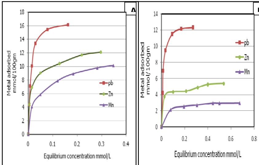
Figure 3: Adsorption isotherms of (A) mono-metal and (B) ternary-metal on apatite mineral at pH (6)
