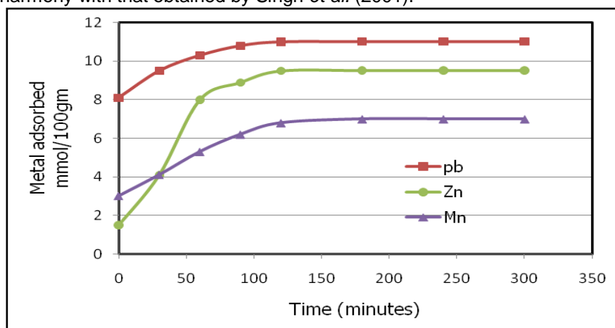
Figure 2: Adsorbed amount of studied heavy metals as a function of time
