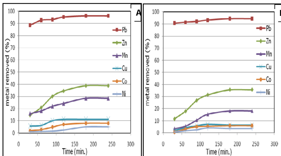
Figure 1: Percentage of ions removed from wastewater by apatite mineral (A) (P1) and (B) (P2)
