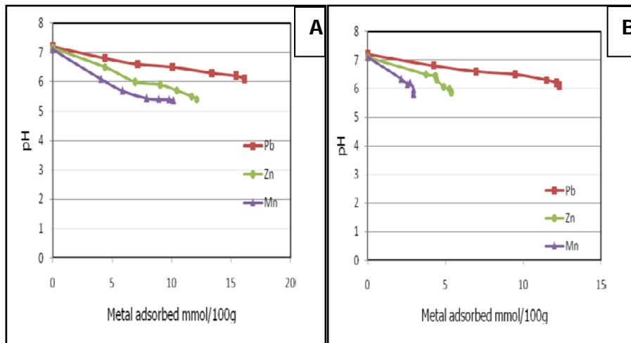
Figure 7: Final pH as a function of metal adsorbed mmol/100g free control system (A) mono-metal (B) ternary-metal
